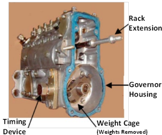
Pump with Existing Governor Housing. Rack Extension Installed
